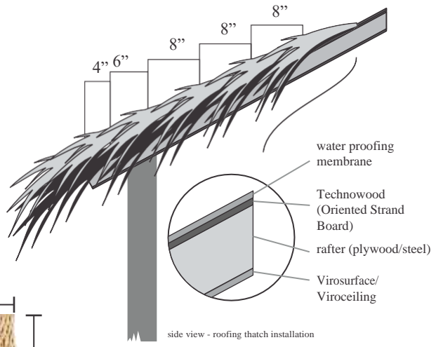
Roofing Thatch Java & Bali stacking 8 inch
